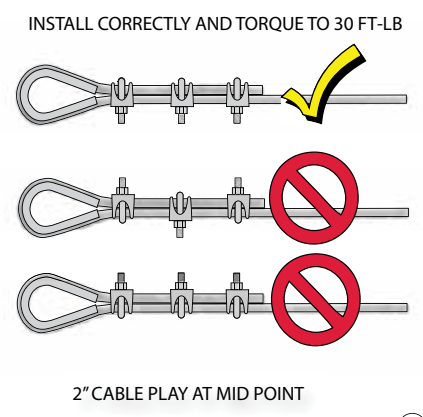
Detail F
